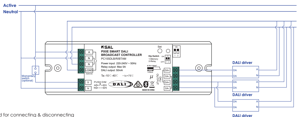
Wiring diagram
