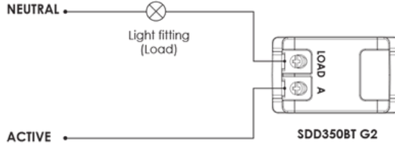
SDD350BT G2 - Standard wiring diagram
